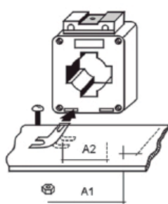
Diagram 1 Fix it with angled flake
