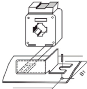
Diagram 2 Fix it on two sides
